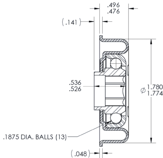
BEARING CROSS SECTION DETAILED VIEW
