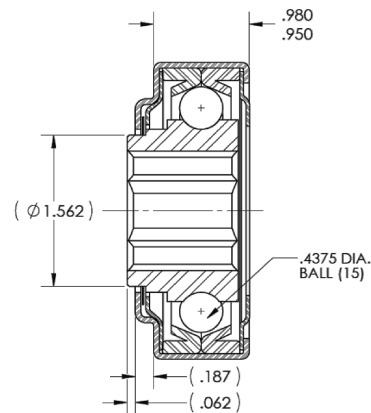
BEARING CROSS SECTION DETAILED VIEW
