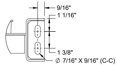
DETAIL A BUTT COUPLING DIMENSIONS
